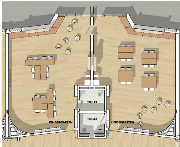
ENLARGED PLAN - TYP KINDERGARTEN/ PRE-K
