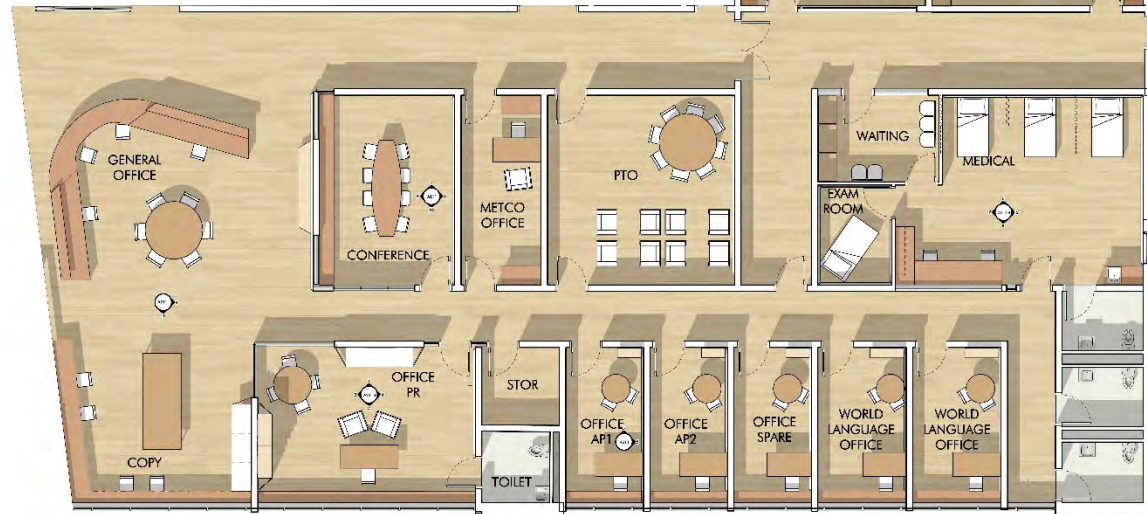
FIRST FLOOR - ADMIN
